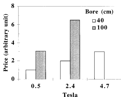
Figure 1. Prices of magnets for different fields and different bore diameters.
